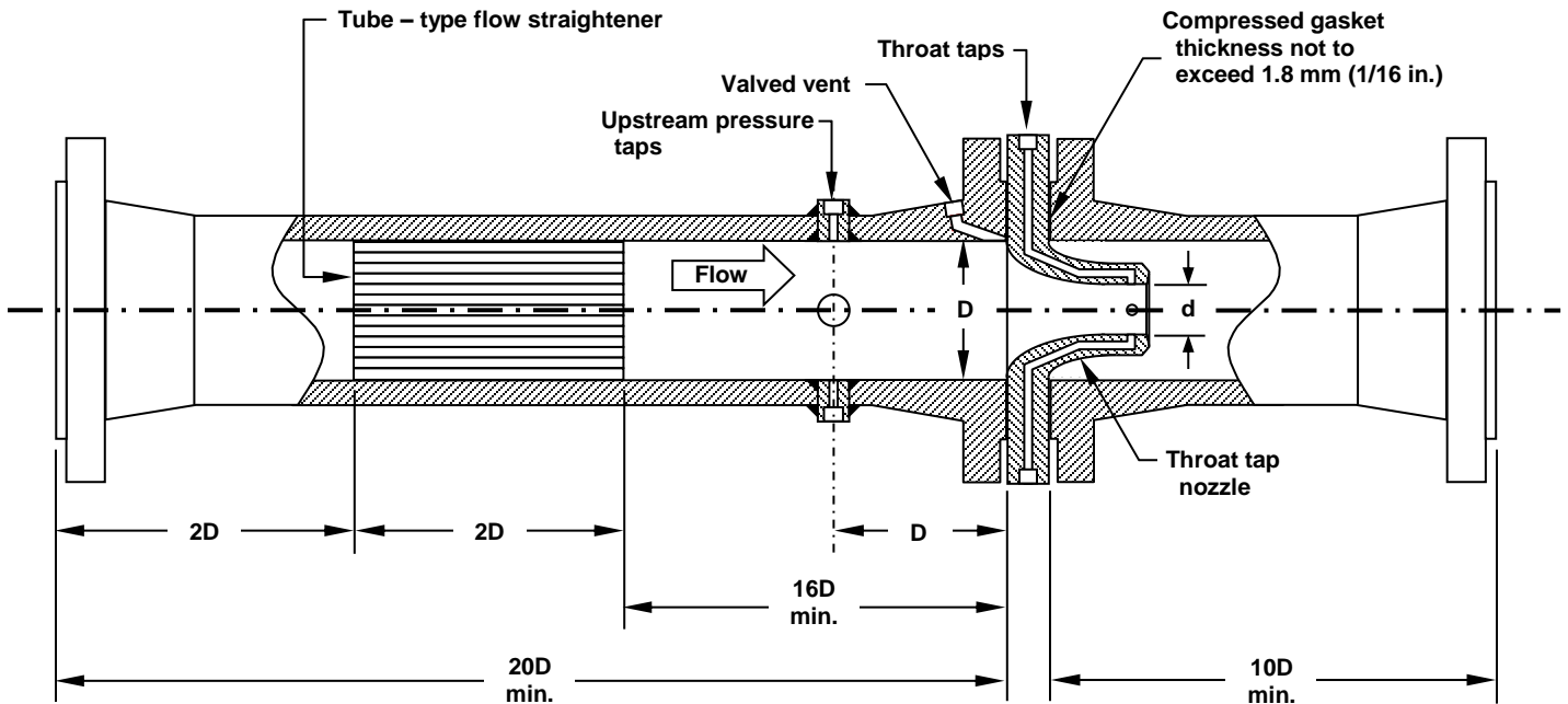
PTC-6 Test Section with Tube-Type Flow Straightener, Model FNP-TS
