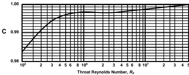
Reference Curve for Nozzle Calibration
